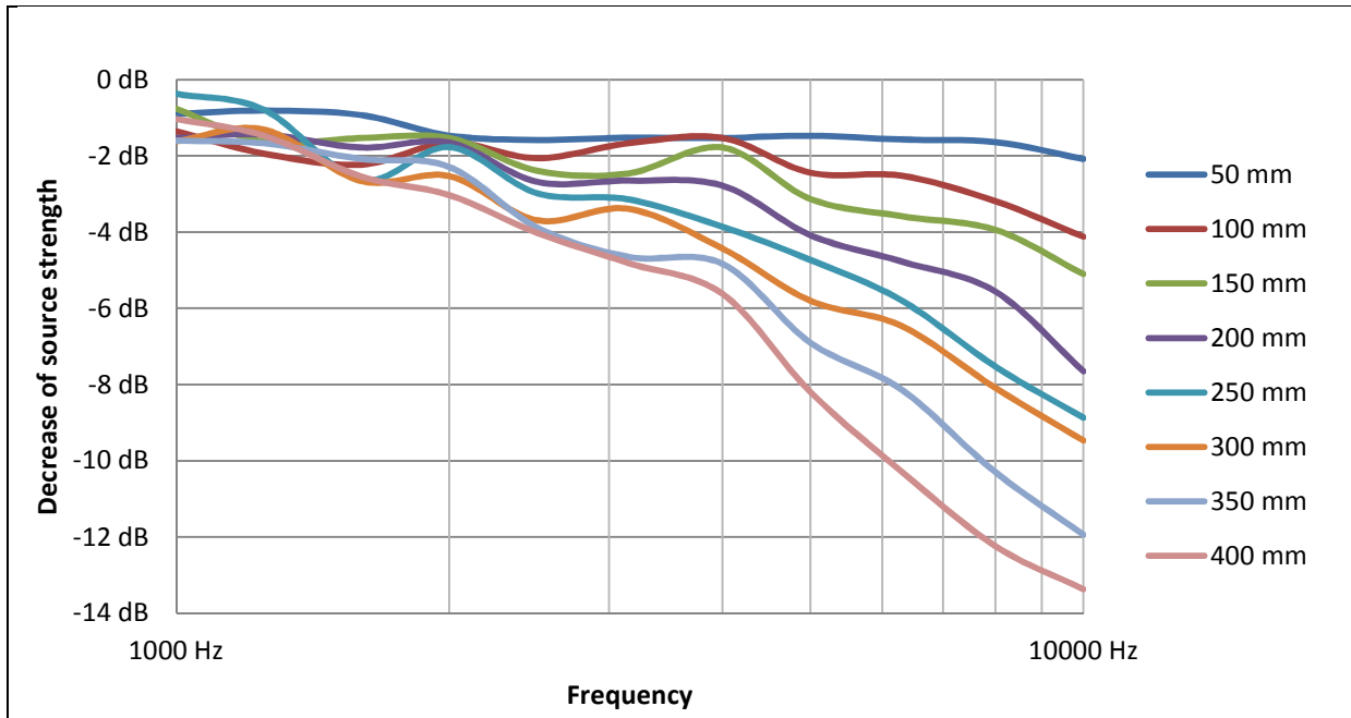
Fig. 11: Source strength in relation to focus deviation and frequency, array 5 m x 3 m, source distance from array 3.5 m
